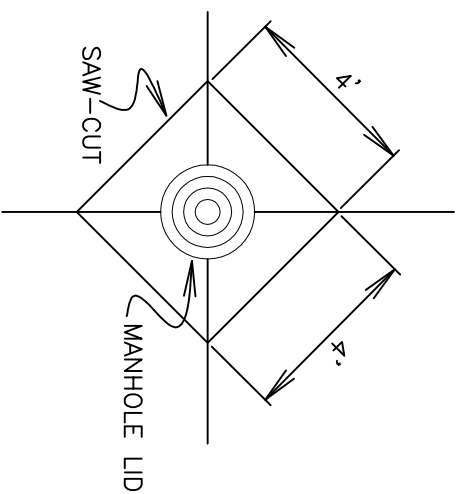
MANHOLE SAW-CUT DETAIL
