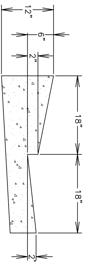
SECTION 3 MOUNTABLE CURB AND GUTTER
