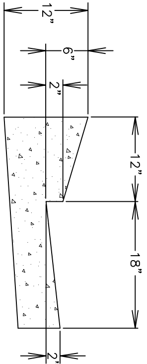
SECTION 2 MOUNTABLE CURB AND GUTTER
