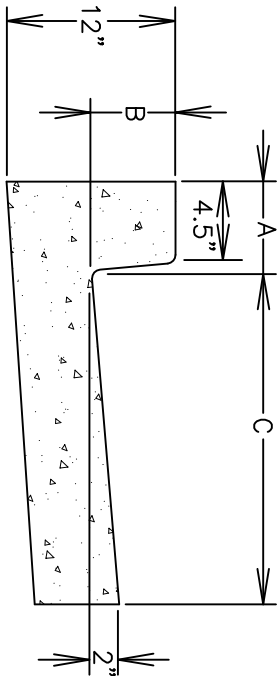
SECTION 1 CURB AND GUTTER
